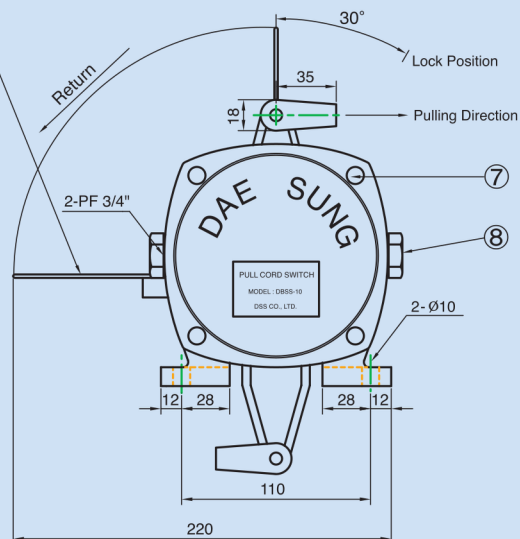
Operating Indicator Plate
